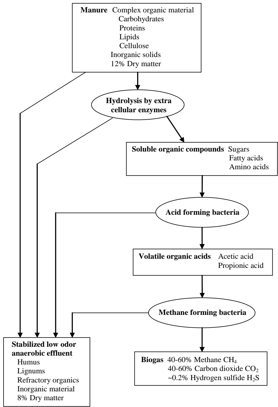
Figure 10. Anaerobic digestion of dairy manure.
